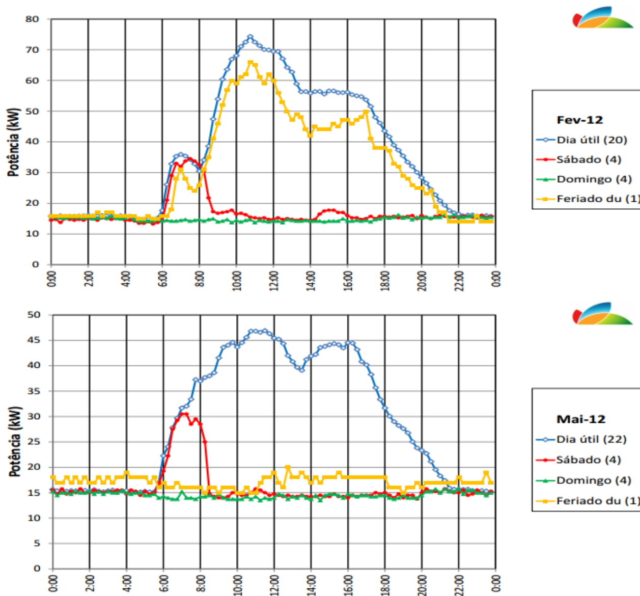
Figure 17: Energy consumption paths changes through behaviour change in energy consumption
